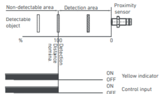
Operating diagram
