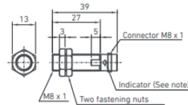
M8x1 inductive detector with M8x1 connector
