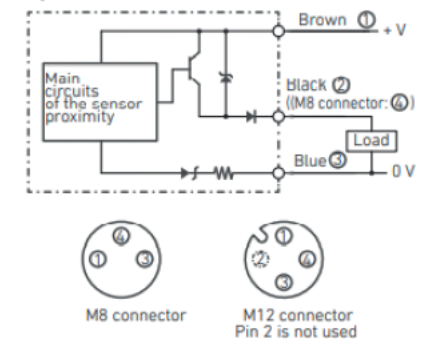
Input circuit
