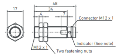
Inductive detector M12x1 with connector M12x1
