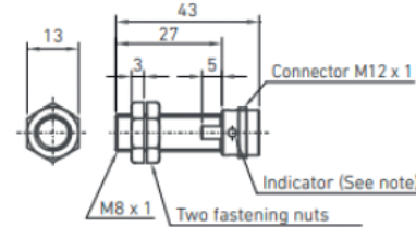
Inductive detector M8x1 with connector M12x1 (optional)
