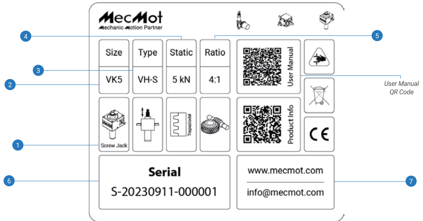
*Example of MecMot Screw Jack Rating Plate
